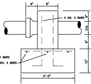
RESTRAINING COLLAR CONCRETE PIER
