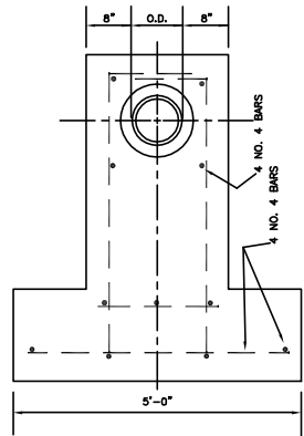
STANDARD CONCRETE PIER
