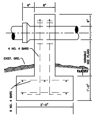
STANDARD CONCRETE PIER
