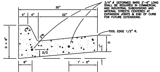
COMBINED CURB & GUTTER DETAIL
