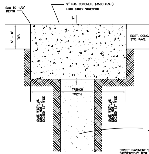
P.C. CONCRETE STREET & ALLEY PAVEMENT
