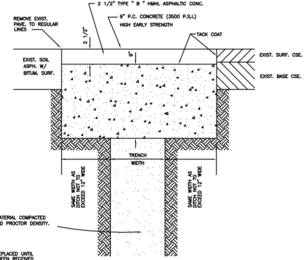
BITUMINOUS STREET & ALLEY PAVEMENT
