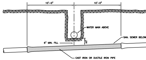
SANITARY SEWER CROSSING
