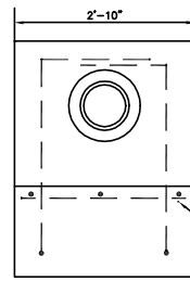
RESTRAINING COLLAR CONCRETE PIER
