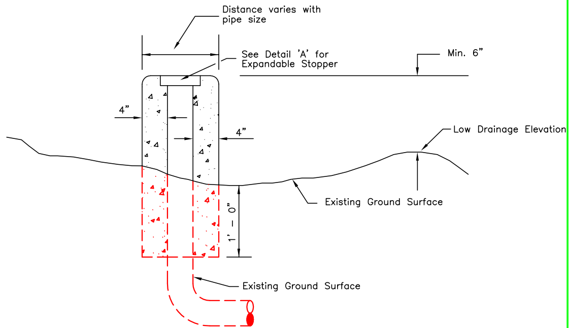
SIDE VIEW Not To Scale
